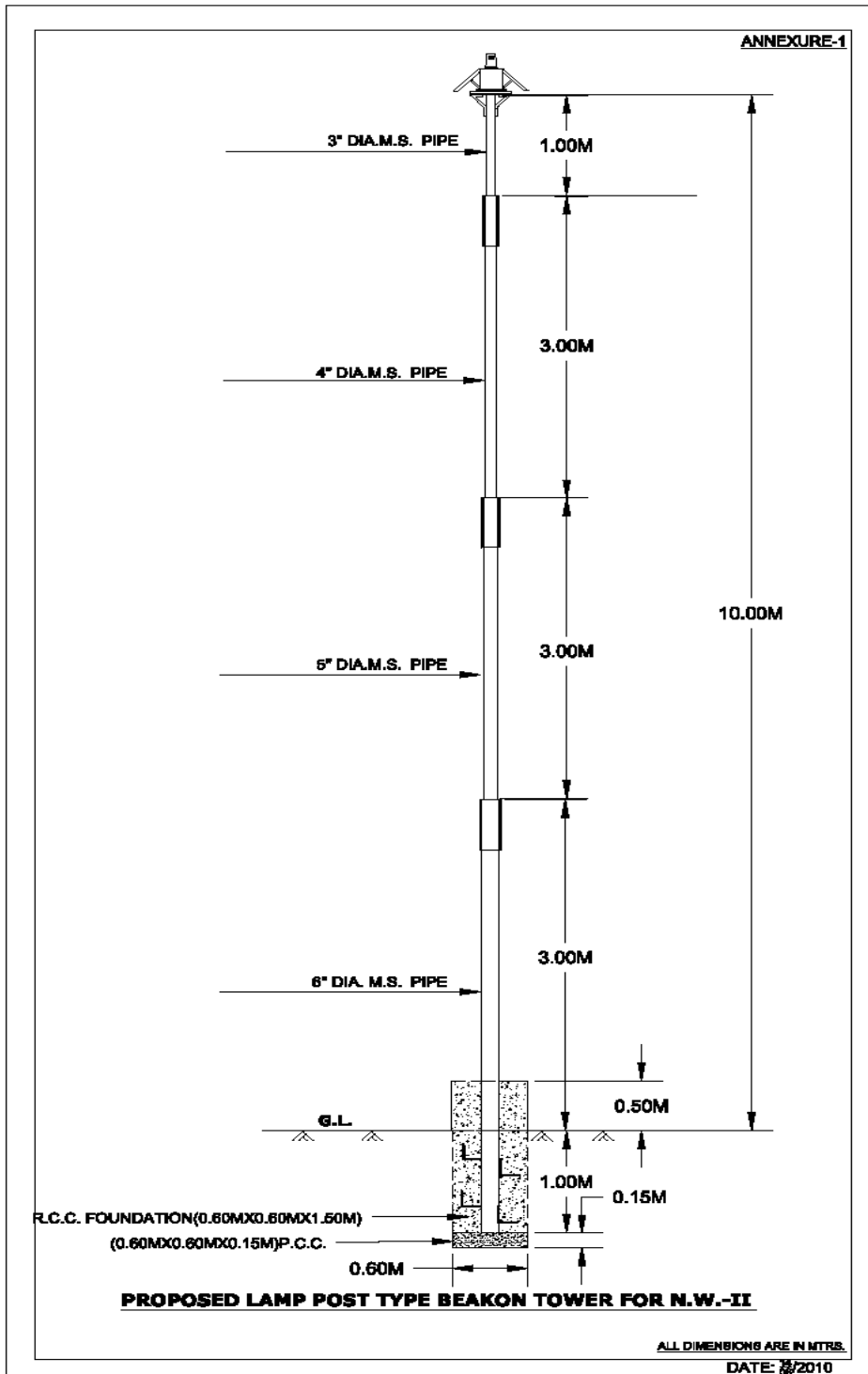
DRAWING OF BEACON TOWER WITH M.S.PIPE
